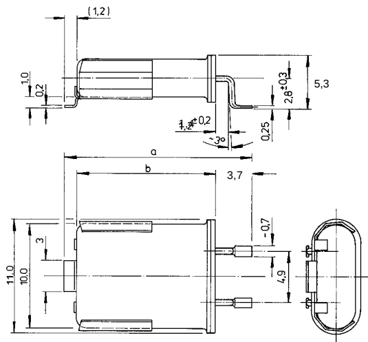
Crystal enclosure HC-49-SMD
